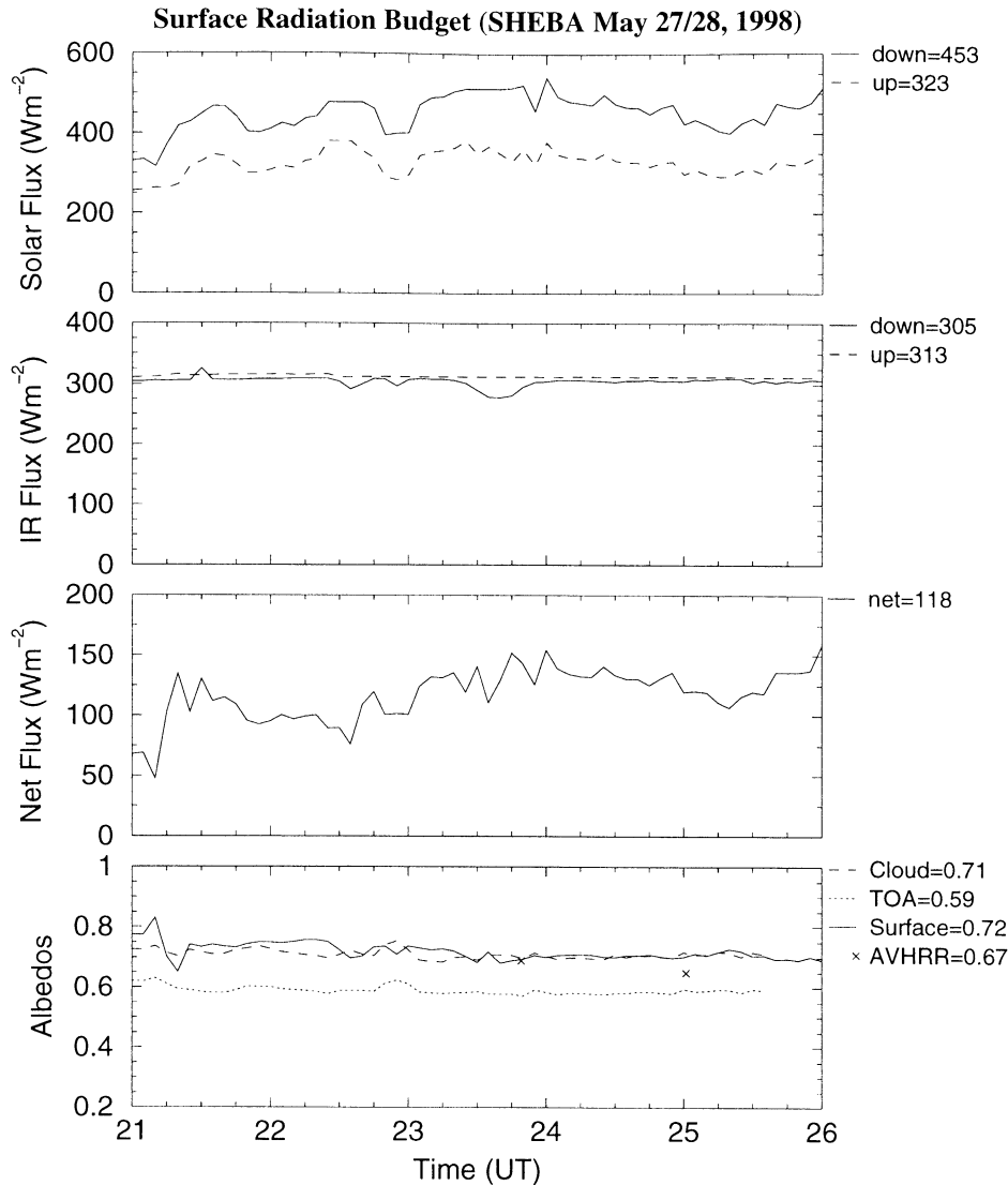
Figure 10. Same as Figure 8 but for Case 3.
