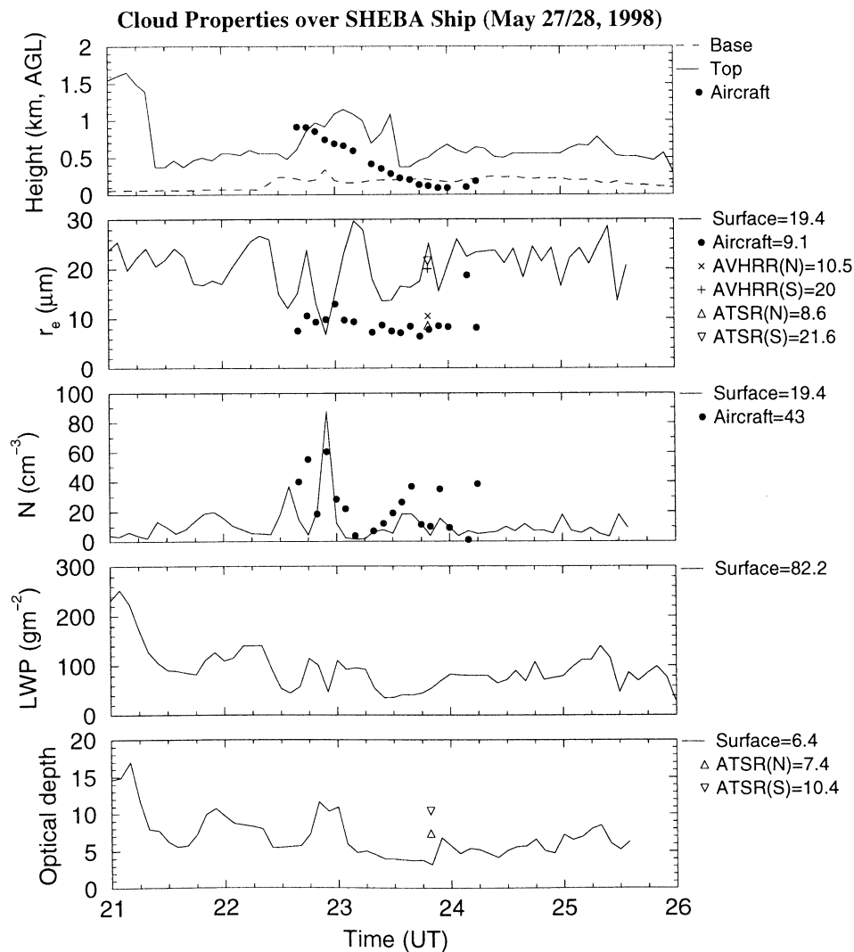
Figure 4. Same as Figure 2 but for Case 3. The satellite results are shown in the north of the ship with N and the south of the ship with S .
