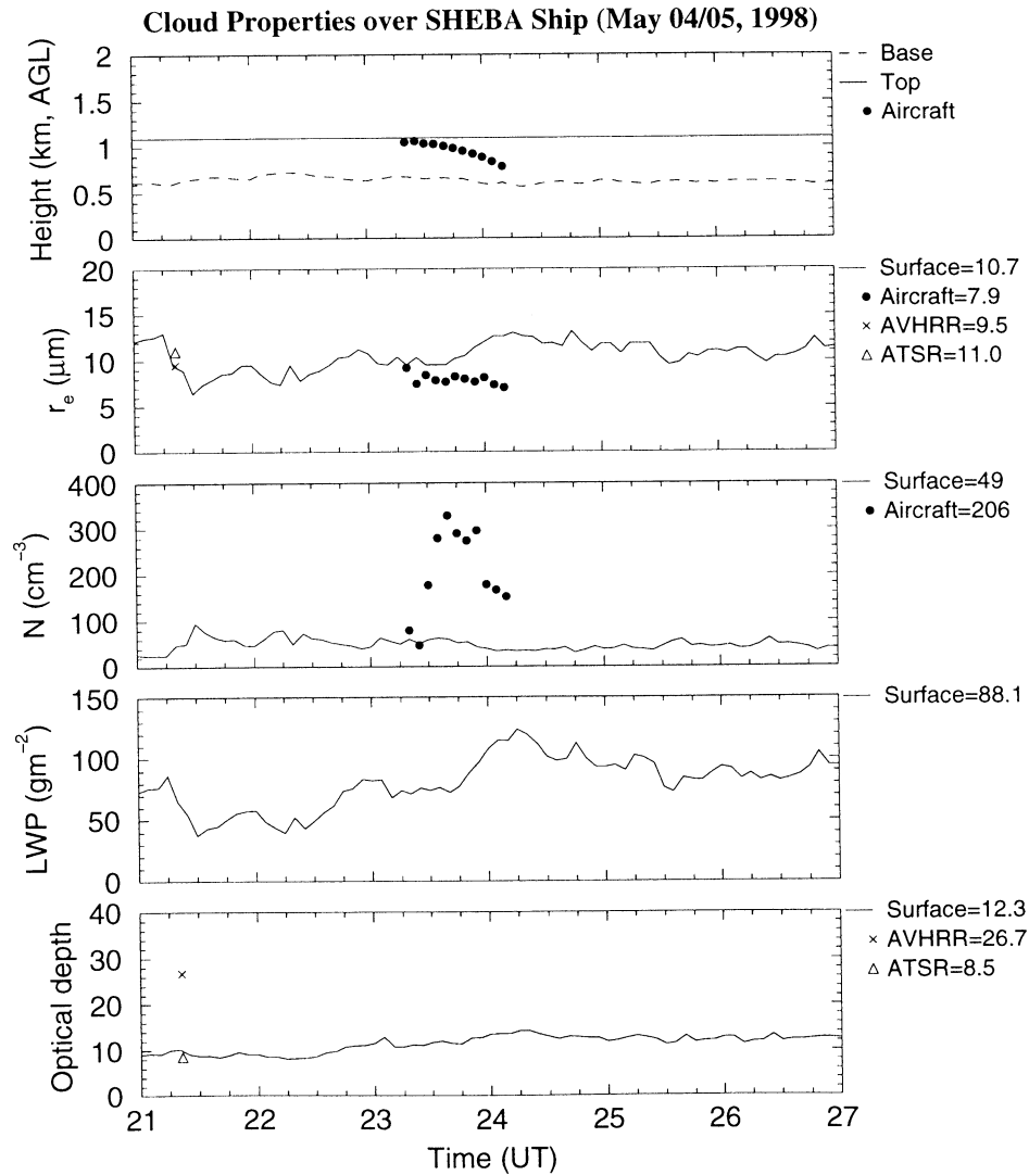
Figure 2. Cloud top height from the 35 GHz cloud radar (fixed at 1.1 km in this case), cloud base height from the laser ceilometer, and cloud liquid water path LWP from the microwave radiometer. The cloud-droplet effective radius r_e , number concentration N , and optical depth \tau were retrieved from the \delta 2 -stream model. The aircraft values of r_e and N were measured by the FSSP-100. Satellite results were retrieved from VISTB; 2400 UT corresponds to 0000 UT, May 5.
