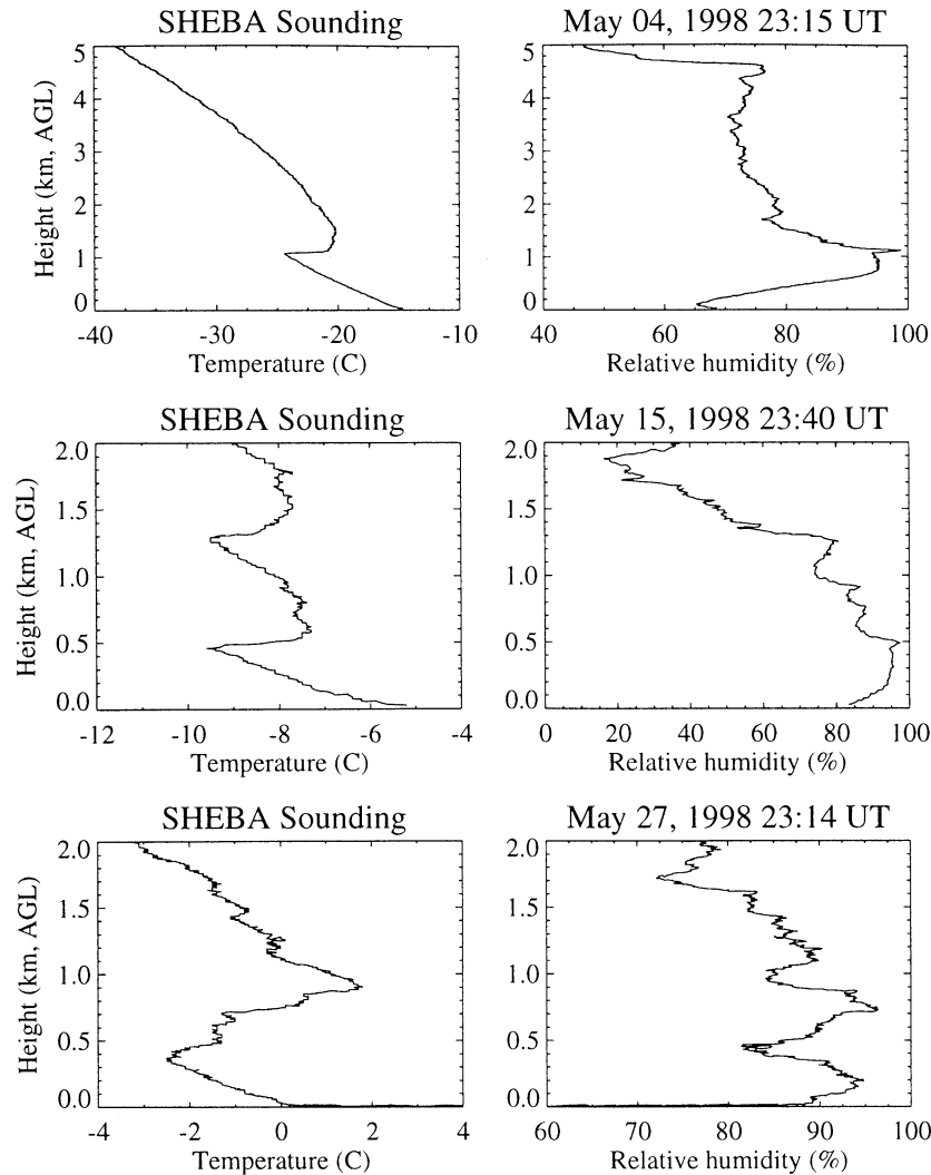
Figure 1. Three cloudy soundings were launched around local noon (2300 UT) from SHEBA ship at the locations of 76.013°N/165.357°W (May 4, Case 1), 76.297°N/165.271°W (May 15, Case 2), and 76.556°N/168.004°W (May 27, Case 3), respectively.
