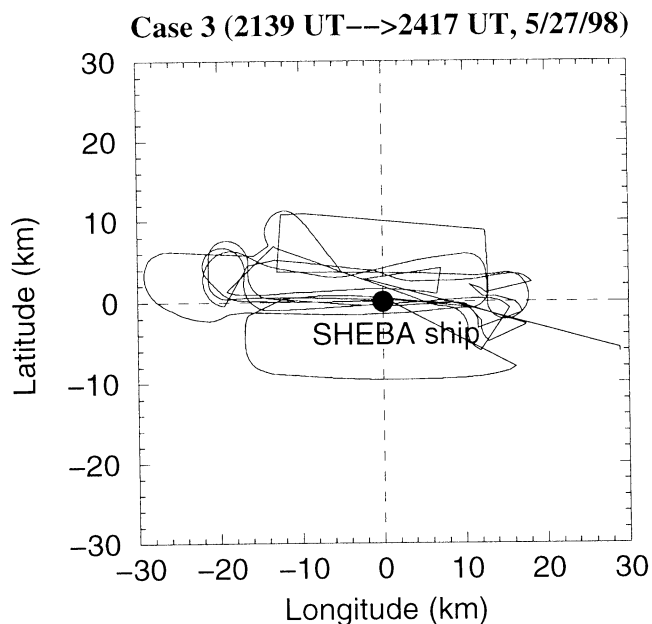
Figure 7. NCAR C-130Q research aircraft flight patterns over the SHEBA ship during the May 27/28, 1998, Case 3.
