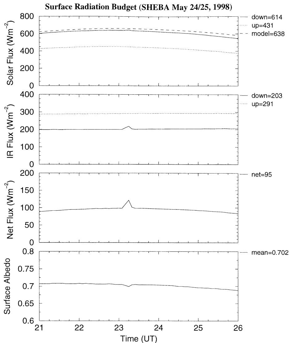
Figure 12. Same as Figure 11 but for another clear-sky day.
