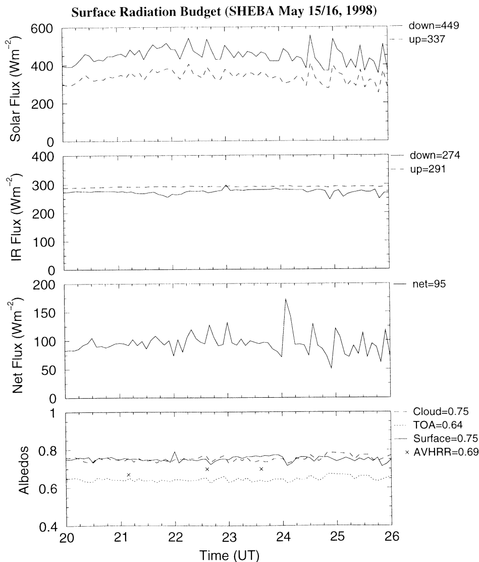
Figure 9. Same as Figure 8 but for Case 2.
