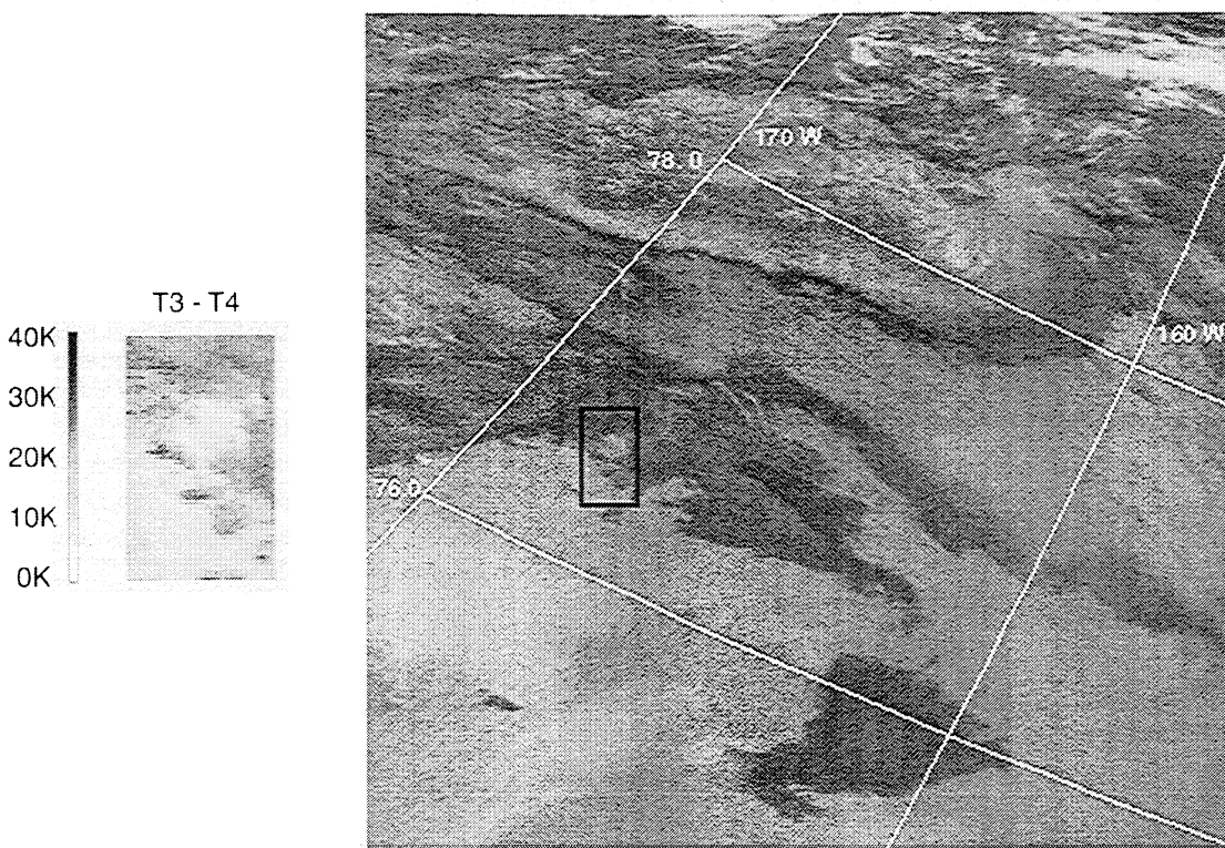
Figure 5. The 3.75 \mu\text{m} (T3) and its temperature difference with 10.8 \mu\text{m} (T4) images from the NOAA-14 overpass at 2349 UT, May 27, 1998. The SHEBA ship is the center of the 20 \times 20 \text{ km} box.
