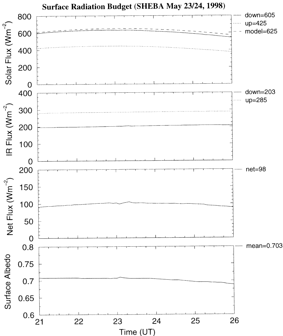
Figure 11. Same as Figure 8 but for clear-sky conditions. The modeled downward solar flux at the surface was calculated from the \delta 2 -stream model with the input of measured surface albedo and sounding.
