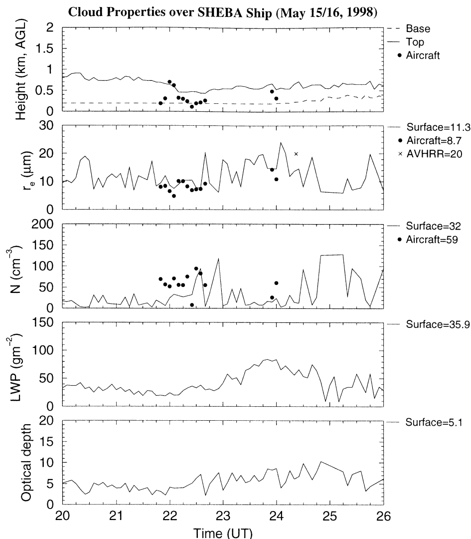
Figure 3. Same as Figure 2 but for Case 2, and the cloud base height was fixed at 0.2 km based on the lidar image because the ceilometer measurement was not available on May 15.
