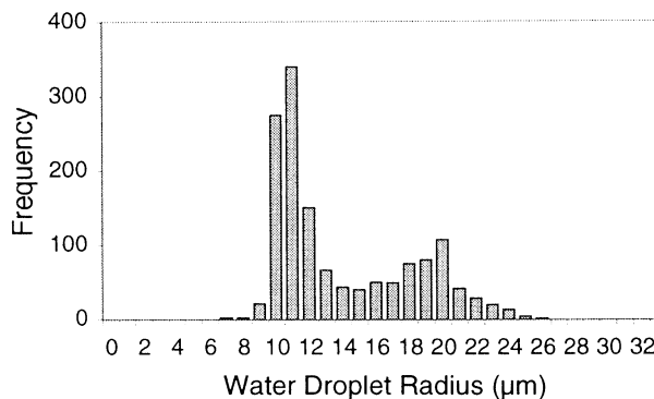
Figure 6. VISTB-retrieved r_e histogram shows that there are two distinct cloud types around the ship. The effective radii in the south of the ship are twice as large as those in the north of the ship.
