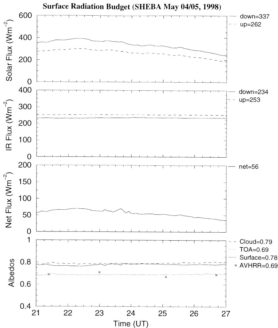
Figure 8. Broadband downward/upward solar and infrared fluxes at the surface were measured by uplooking/downlooking standard Eppley precision spectral radiometers. The cloud and TOA albedos are derived from the \delta 2 -stream model. Satellite-derived broadband TOA albedos are calculated from the empirical relationship between a narrow band and a broad band on the basis of AVHRR-measured visible reflectance.
