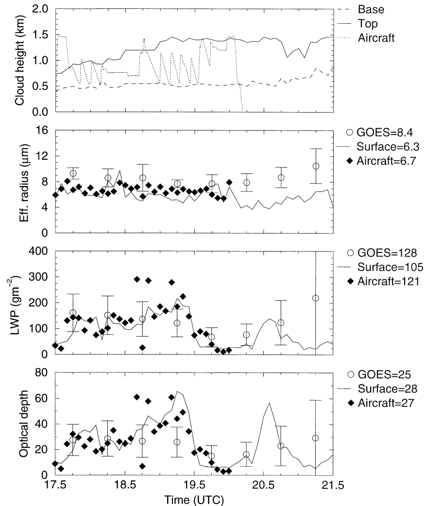
FIG. 4. The ceilometer-measured cloud-base height (dash) and radar-derived cloud-top height (solid), r_e , LWP, and \tau vs time for 3 Mar 2000. The means given on the right of the panels represent the averaged values when all three datasets are available, such as from 17.5 to 20.0 UTC.
